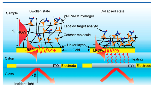
Figure 2. Sensor chip with embedded ITO microheater and SPR-active layer architecture on the top carrying a thermoresponsive pNIPAAm hydrogel layer.
